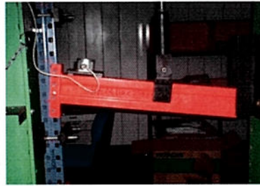
Joint Stiffness test on Beam end connector – Godrej.
